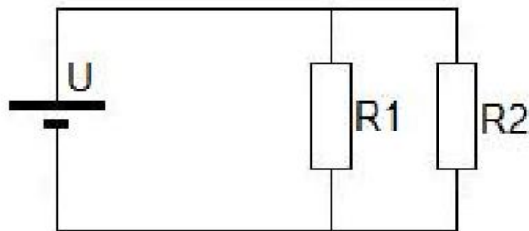
Figur 7.5: Parallellkobling
